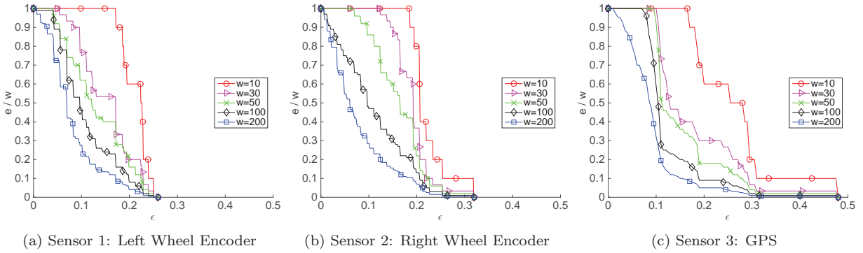
Figure 7: Empirical plots of the proportion of faults in a window ( e/w ) against the error bound ( \epsilon ).
